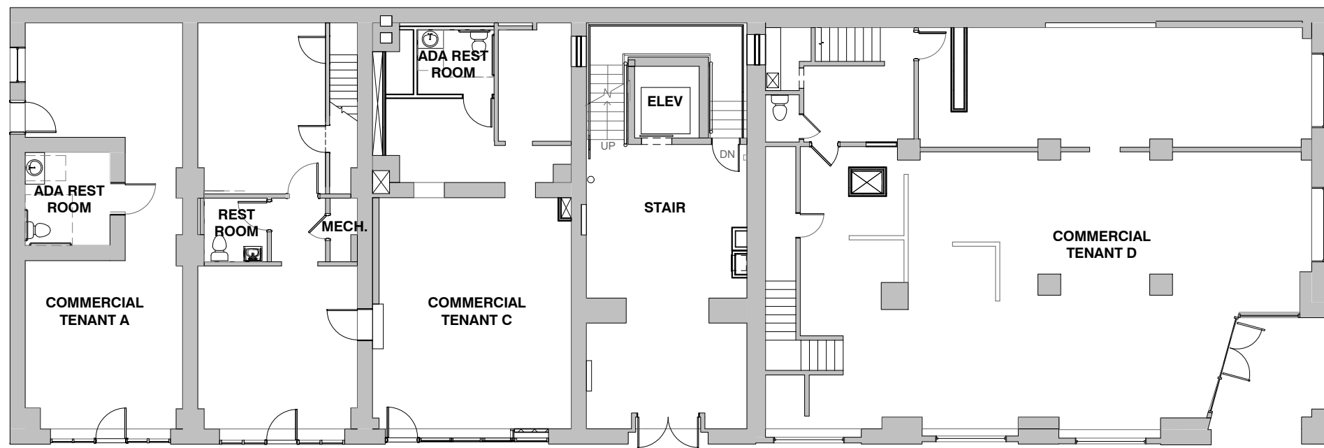
FIRST FLOOR
